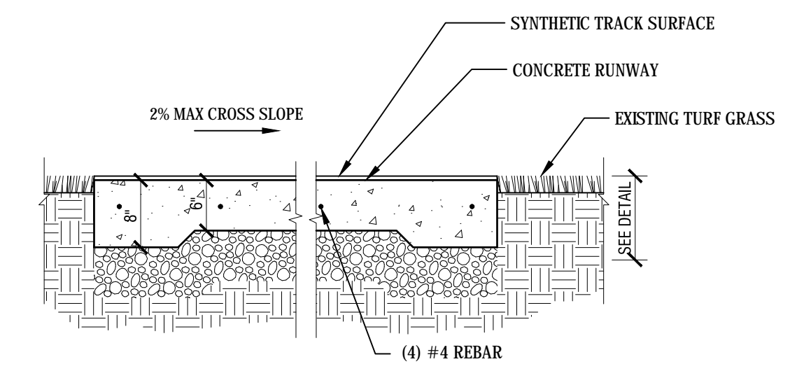
7 RUNWAY CROSS SECTION AT LONG JUMP 3/4" = 1'-0"
