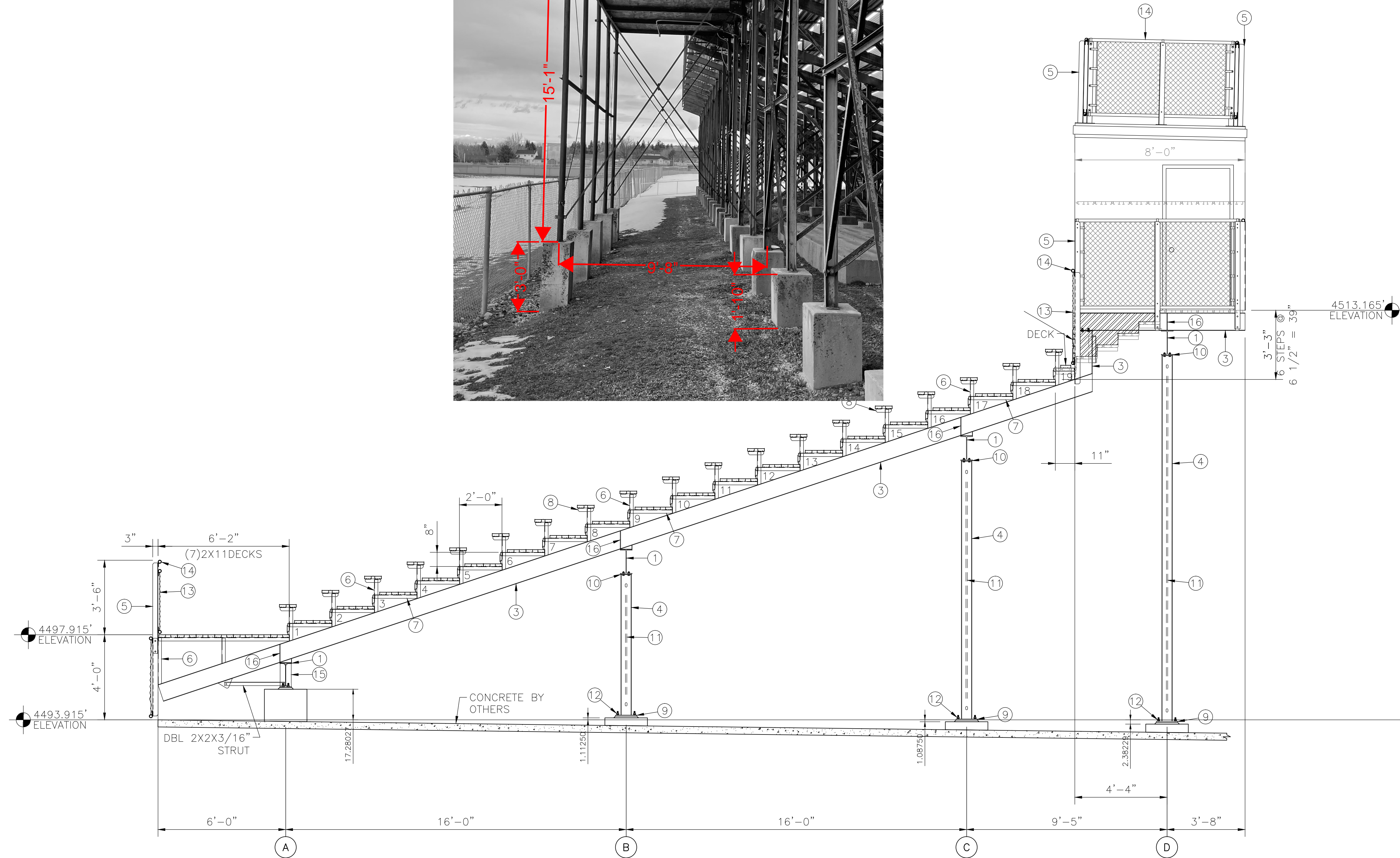
SECTION VIEW @ PRESSBOX SCALE: 3/8" = 1'-0"
